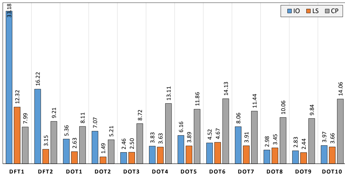
Figure 6. PF_E (%) for optimally designed 10-story SCBFs at IO, LS and CP performance levels
