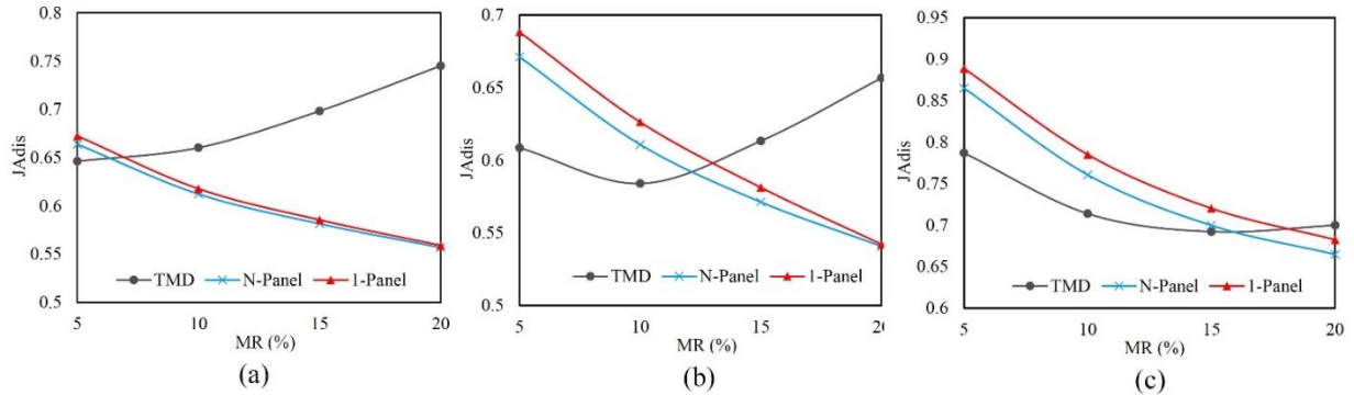
Figure 6. Optimum values of displacement objective function for different MRs (a) 10-story model (b) 20-story model (c) 30-story model
